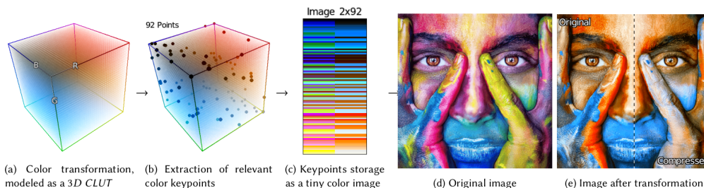
Figure 5: G'MIC color LUT compression: a CLUT (a) is analyzed, relevant keypoints are deduced and stored (b,c). A perceptual metric ensure that the difference between original/compressed CLUTs are imperceptible.
